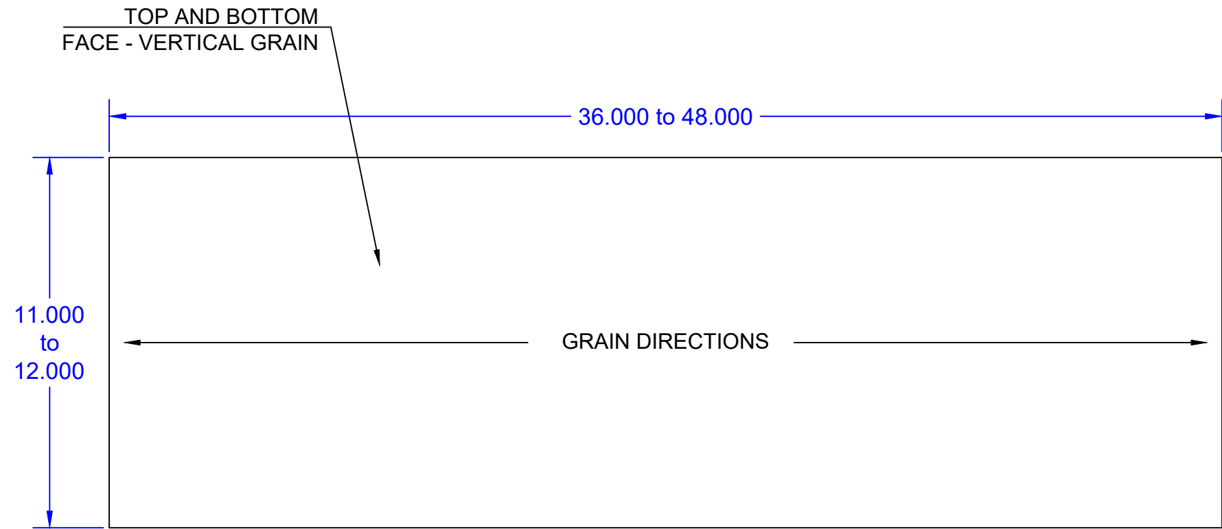
TOP VIEW:
